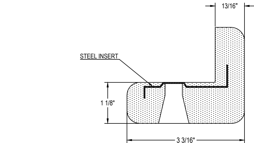
CROSS SECTION
